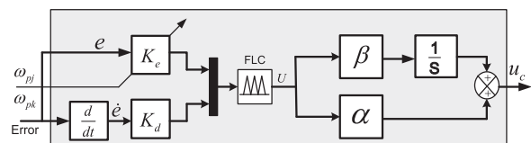
Fig. 7. Simulink model of fuzzy PID type controller.
